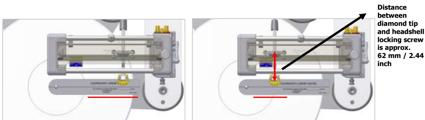
Pic.18: Adjustment of the linear tracking
